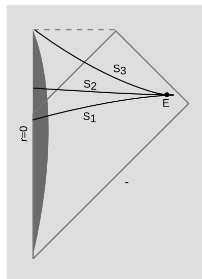
e / According to the distant observer, does the infalling matter ever reach the singularity?
