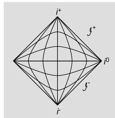
a / Penrose diagram for flat spacetime.
