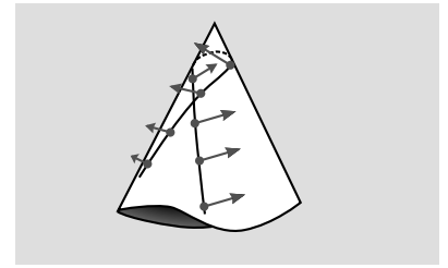
b / The cone has zero intrinsic curvature everywhere except at its tip. An observer who never visits the tip can nevertheless detect its existence, because parallel transport around a path that encloses the tip causes a vector to change its direction.
