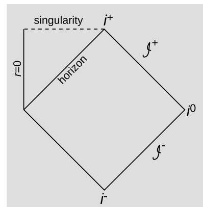
c / Penrose diagram for Schwarzschild spacetime: a black hole that didn't form by gravitational collapse.
