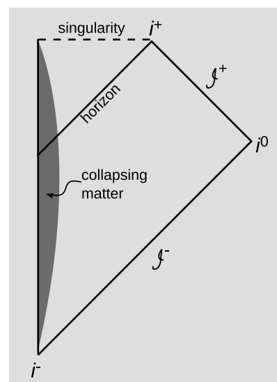
d / Penrose diagram for a black hole formed by gravitational collapse.
