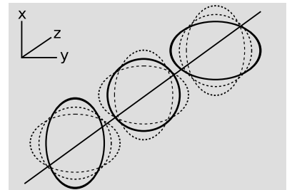
f / As the gravitational wave propagates in the z direction, the metric oscillates in the x and y directions, preserving volume.
