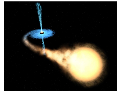
a / A black hole accretes matter from a companion star.
