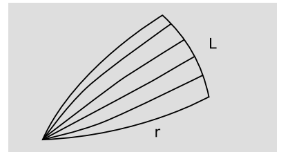
i / 2. Gaussian curvature as L \neq r\theta .
