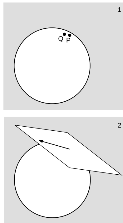
g / 1. A tangent vector can be thought of as an infinitesimal displacement. 2. For a sphere embedded in three-space, the space of tangent vectors is visualized as a plane tangent to the sphere at a certain point.
