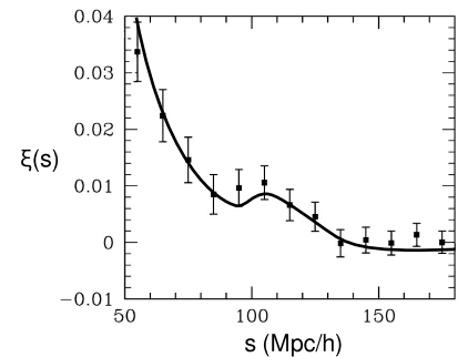
h / The acoustic peak in the BAO correlation function. Redrawn from Eisenstein, New Astronomy Reviews . 49 (2005) 360, as reproduced in Bassett and Hlozek, 2009, arxiv.org/abs/0910.5224 .
