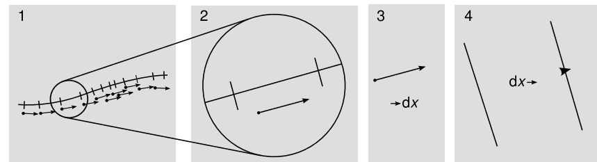
b / The vectors \rightarrow dx and dx \rightarrow are duals of each other.
