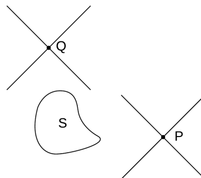
b / Given a finite region of spacetime S, we can find a point like P that is spacelike with respect to the whole region, and a point like Q that is timelike with respect to the whole region.
