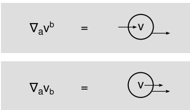
e / Birdtracks notation for the covariant derivative.
