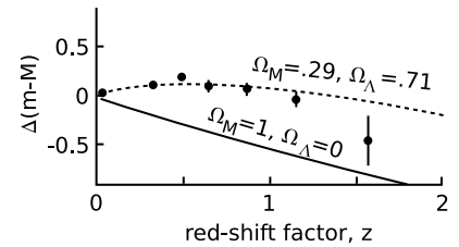
g / A Hubble plot for distant supernovae. Each data point represents an average over several different supernovae with nearly the same z .
