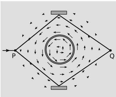
a / The Aharonov-Bohm effect. An electron enters a beam splitter at P, and is sent out in two different directions. The two parts of the wave are reflected so that they reunite at Q. The arrows represent the vector potential A . The observable magnetic field B is zero everywhere outside the solenoid, and yet the interference observed at Q depends on whether the field is turned on. See page 137 for further discussion of the A and B fields of a solenoid.
