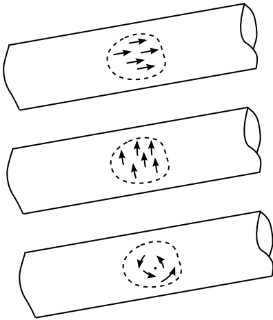
d / Example 3: A cylinder has three local symmetries, but only two that can be extended globally to make Killing vectors.
