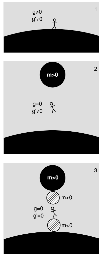
h / Nulling out a gravitational field is impossible in one dimension without exotic matter. 1. The planet imposes a nonvanishing gravitational field with a nonvanishing gradient. 2. We can null the field at one point in space, by placing a sphere of very dense, but otherwise normal, matter overhead. The stick figure still experiences a tidal force, g' \neq 0 . 3. To change the field’s derivative without changing the field, we can place two additional masses above and below the given point. But to change its derivative in the desired direction — toward zero — we would have to make these masses negative.
