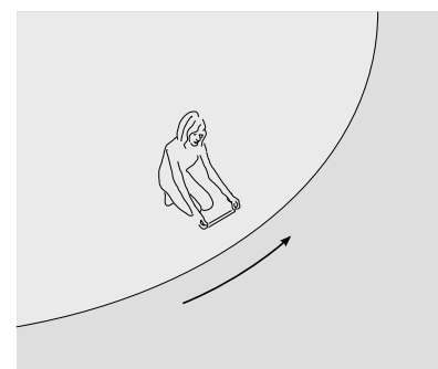
d / Observer A, rotating with the carousel, measures an azimuthal distance with a ruler.
