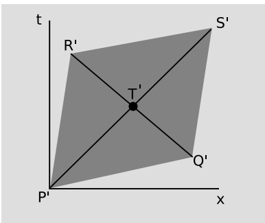
e / Example 8. Flashes of light travel along P'T' and Q'T' . The observer in this frame of reference judges them to have been emitted at different times, and to have traveled different distances.
