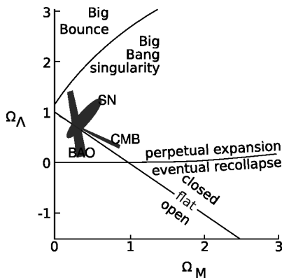
i / The cosmological parameters of our universe, after Perlmutter, 1998, arxiv.org/abs/astro-ph/9812133 and Kowalski, 2008, arxiv.org/abs/0804.4142 . The three shaded regions represent the 95% confidence regions for the three types of observations.
