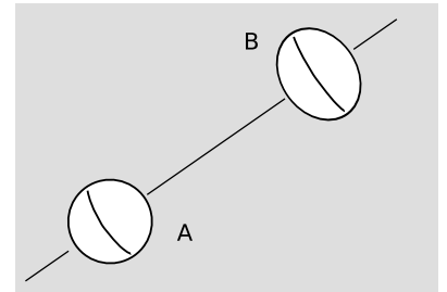
k / One planet rotates about its axis and the other does not. As discussed in more detail on p. 116, Einstein believed that general relativity was even more radically egalitarian about frames of reference than it really is. He thought that if the planets were alone in an otherwise empty universe, there would be no way to tell which planet was really rotating and which was not, so that B’s equatorial bulge would have to disappear. There would be no way to tell which planet’s surface was a Lorentz frame.
