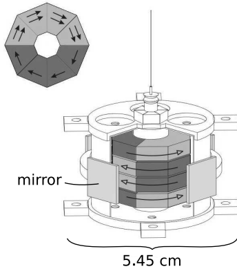
d/The University of Washington torsion pendulum used to search for torsion. The light gray wedges are Alnico, the darker ones \text{SmCo}_5 . The arrows with the filled heads represent the directions of the electron spins, with denser arrows indicating higher polarization. The arrows with the open heads show the direction of the \mathbf{B} field.
