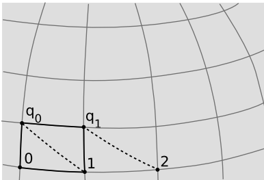
a / Construction of an affine parameter in curved spacetime.
