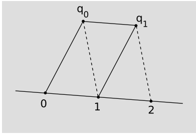
d / Construction of an affine parameter.
